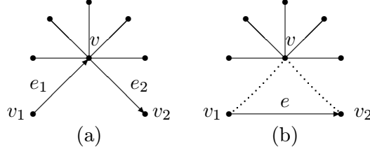
Figure 3.1: Vertex Splitting
