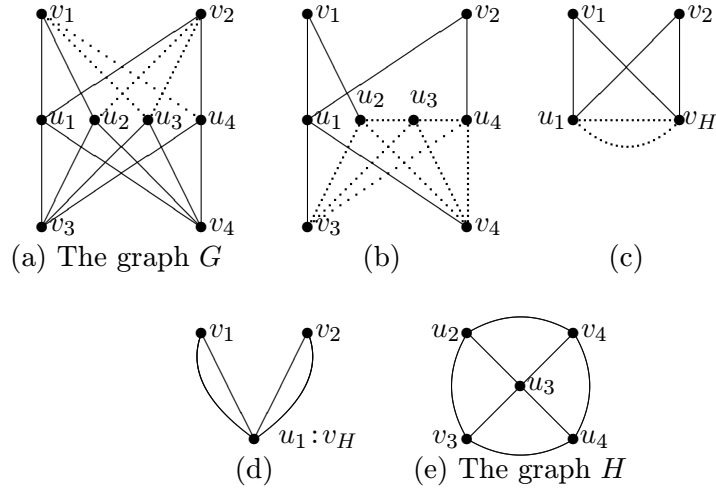
Figure 4.4: Reduction of K_{4,4}
