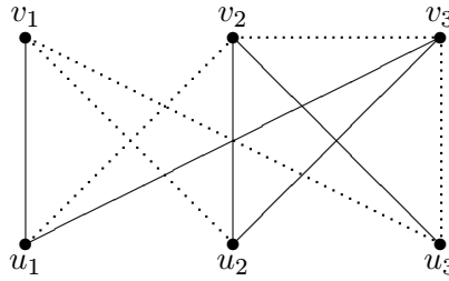
Figure 4.2: K_{3,3}
