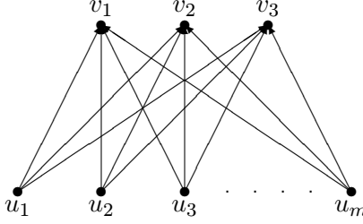
Figure 4.3: K_{m,3}
