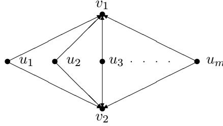
Figure 4.1: K_{m,2}
