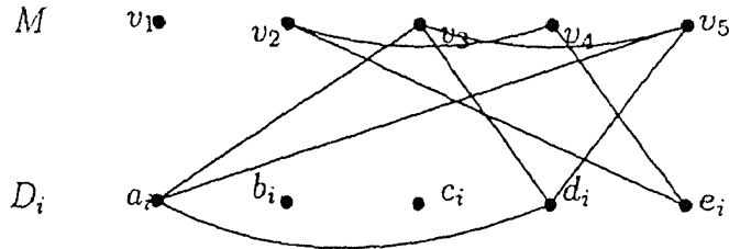
Figure 10. The complement of H_2
