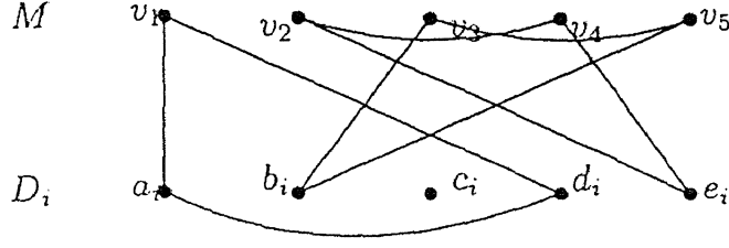
Figure 7. The complement of H_3
